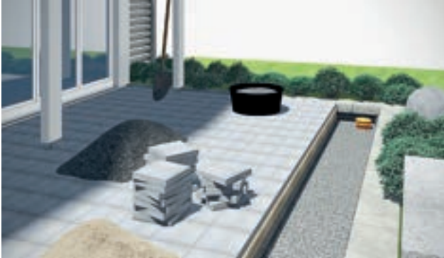
Produce trench in which to lay channel with frost resistant sub base.
